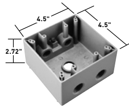
2 Gang Deep Box
