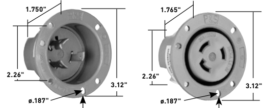
30A Flanged Inlet & Outlet
