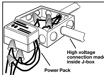
Ceiling Sensor with Power Pack
