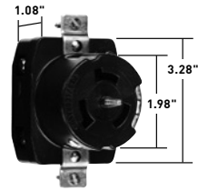
California Standard Receptacle
